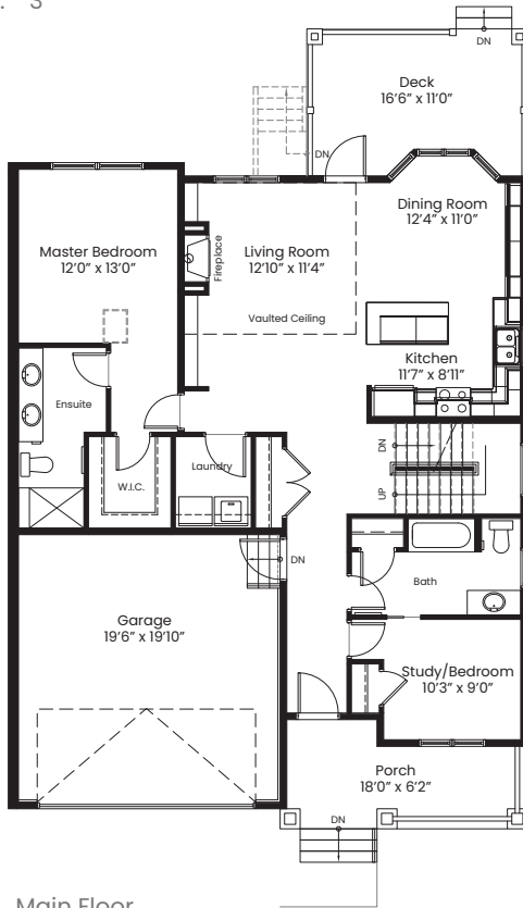
Main Floor 1337 Sq.Ft.
